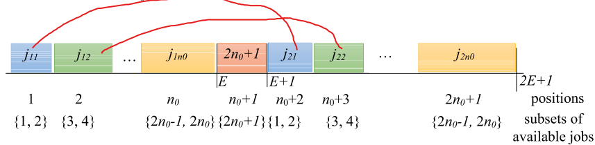
Fig. 1 Illustrative example to the reduction of the Ordered Partition Problem to 1|d_j = d|\sum_j w_j U_j with job prohibitions. Here we present a scheme of a non-idle schedule in which jobs form \{j_{11}, \dots, j_{1n_0}\} complete before time E , jobs form \{j_{21}, \dots, j_{2n_0}\} start after time E and
